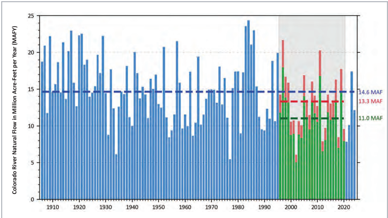
FIGURE 4.5 Water Supply Conditions Evaluated in Planning Scenarios
